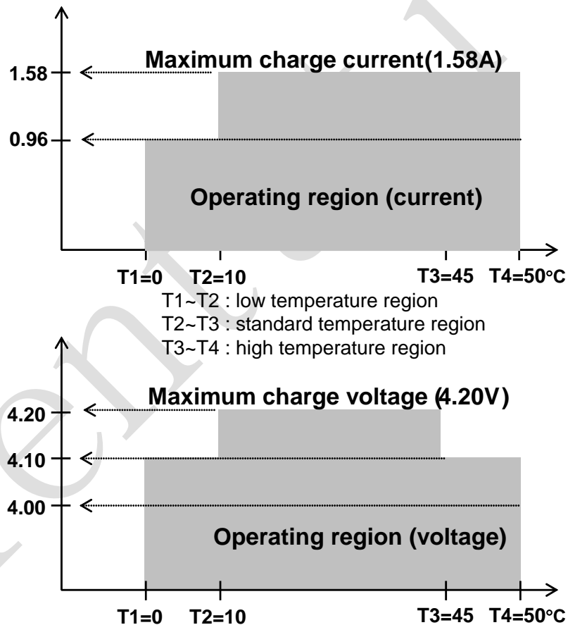
Fig. 1. Charging operating window for reliable cycle life.
